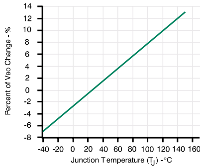
TYPICAL V_{BO} CHANGE vs JUNCTION TEMPERATURE
