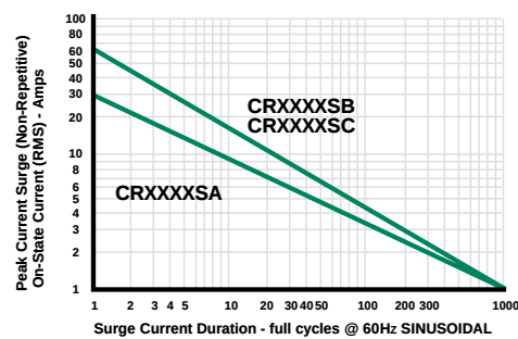
PEAK SURGE ON-STATE CURRENT VS. SURGE CURRENT DURATION
