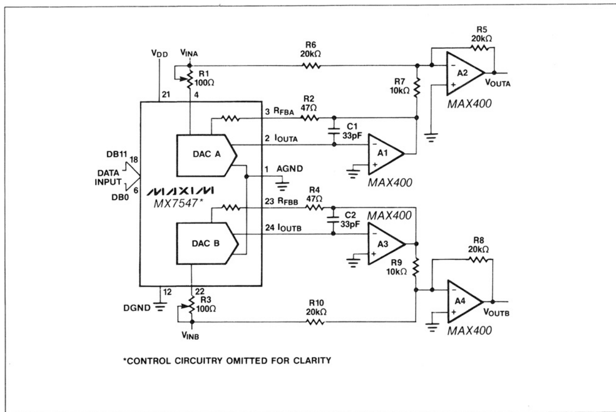
Figure 5B. MX7547 Bipolar Operation (Offset Binary Coding)
