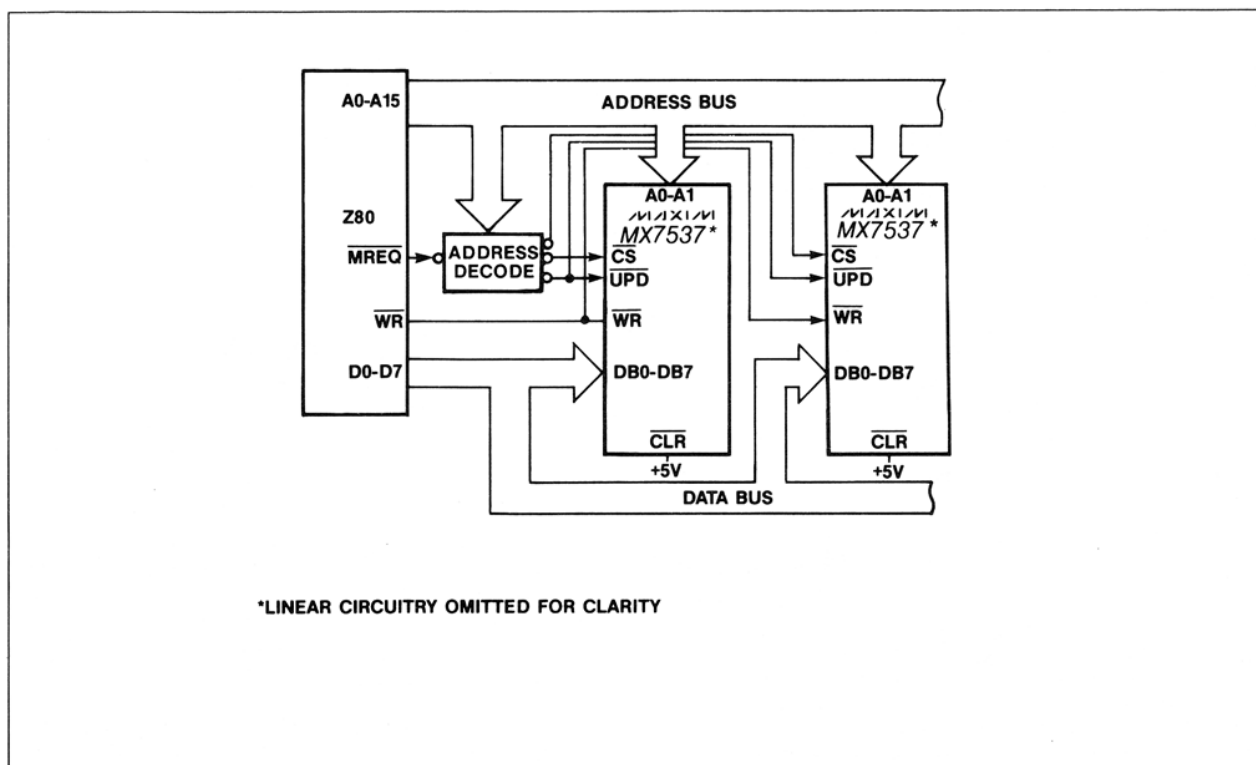
Figure 12. Expanded MX7537 System
