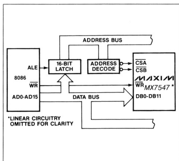
Figure 14. MX7547 — 8086 Interface
