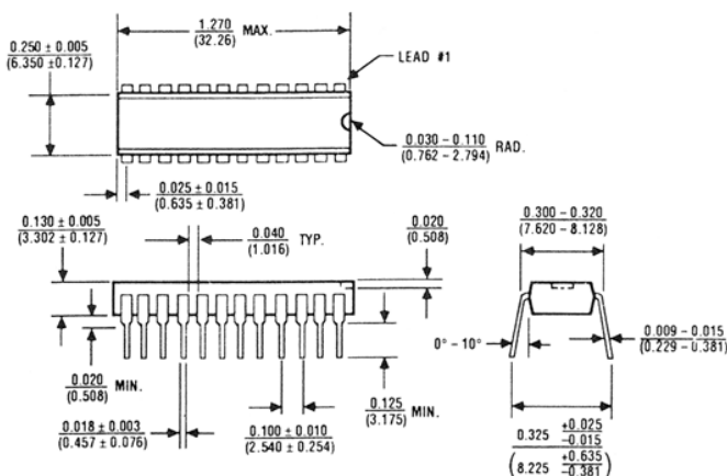
24 Lead Plastic Narrow DIP (NG)
