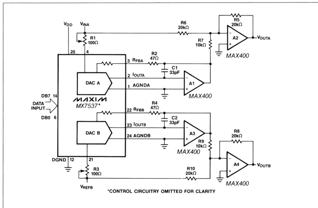
Figure 5A. MX7537 Bipolar Operation (Offset Binary Coding)
