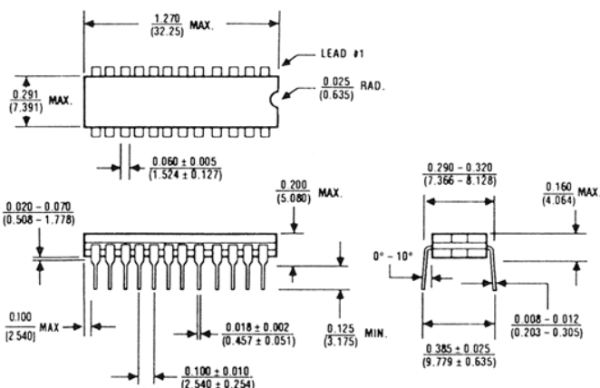
24 Lead Narrow Cerdip (RG)
