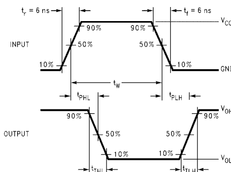
FIGURE 3. AC Waveforms
