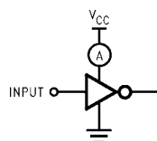
FIGURE 2. I CCD Test Circuit
