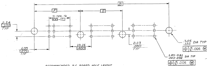
RECOMMENDED P.C. BOARD HOLE LAYOUT
