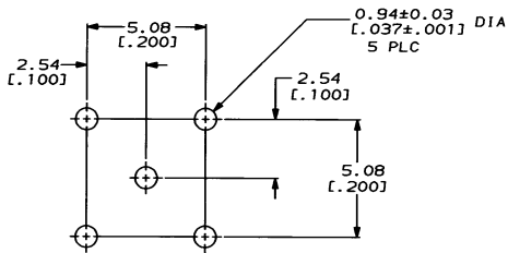
PCB CONFIGURATION
