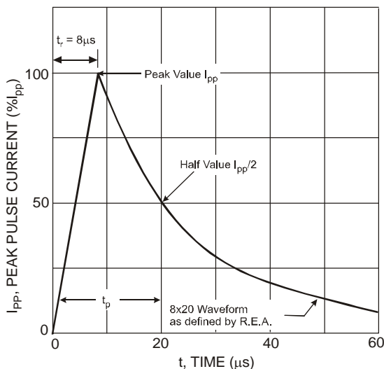
Fig. 1 Pulse Waveform
