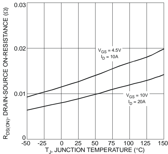
Fig. 10 On-Resistance Variation with Temperature
