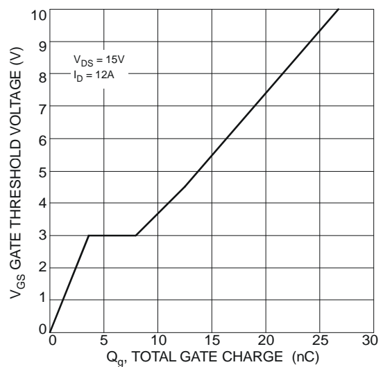
Fig. 15 Gate Charge
