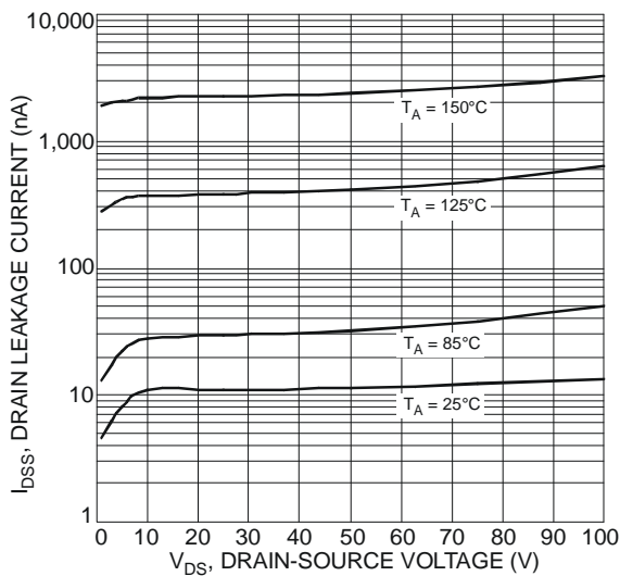
Fig. 14 Typical Drain-Source Leakage Current vs. Voltage
