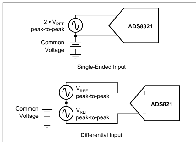
FIGURE 1. Methods of Driving the ADS8321—Single-Ended or Differential.
