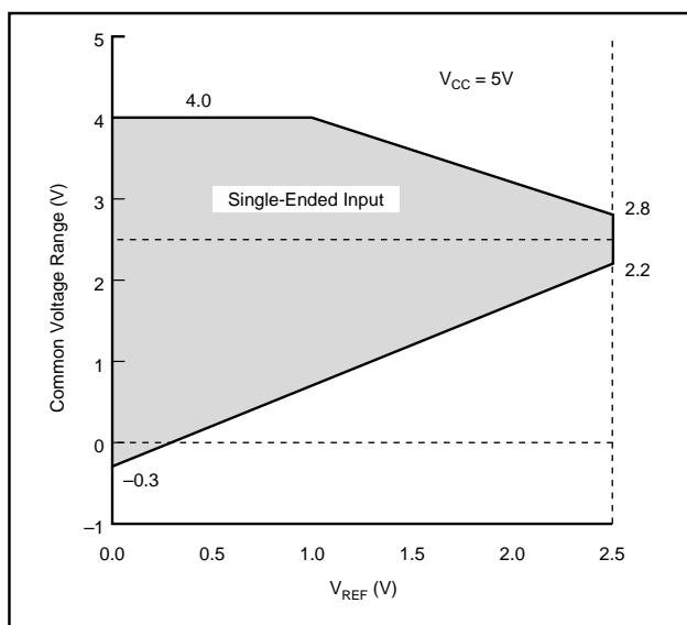
FIGURE 2. Single-Ended Input—Common Voltage Range vs V REF .
