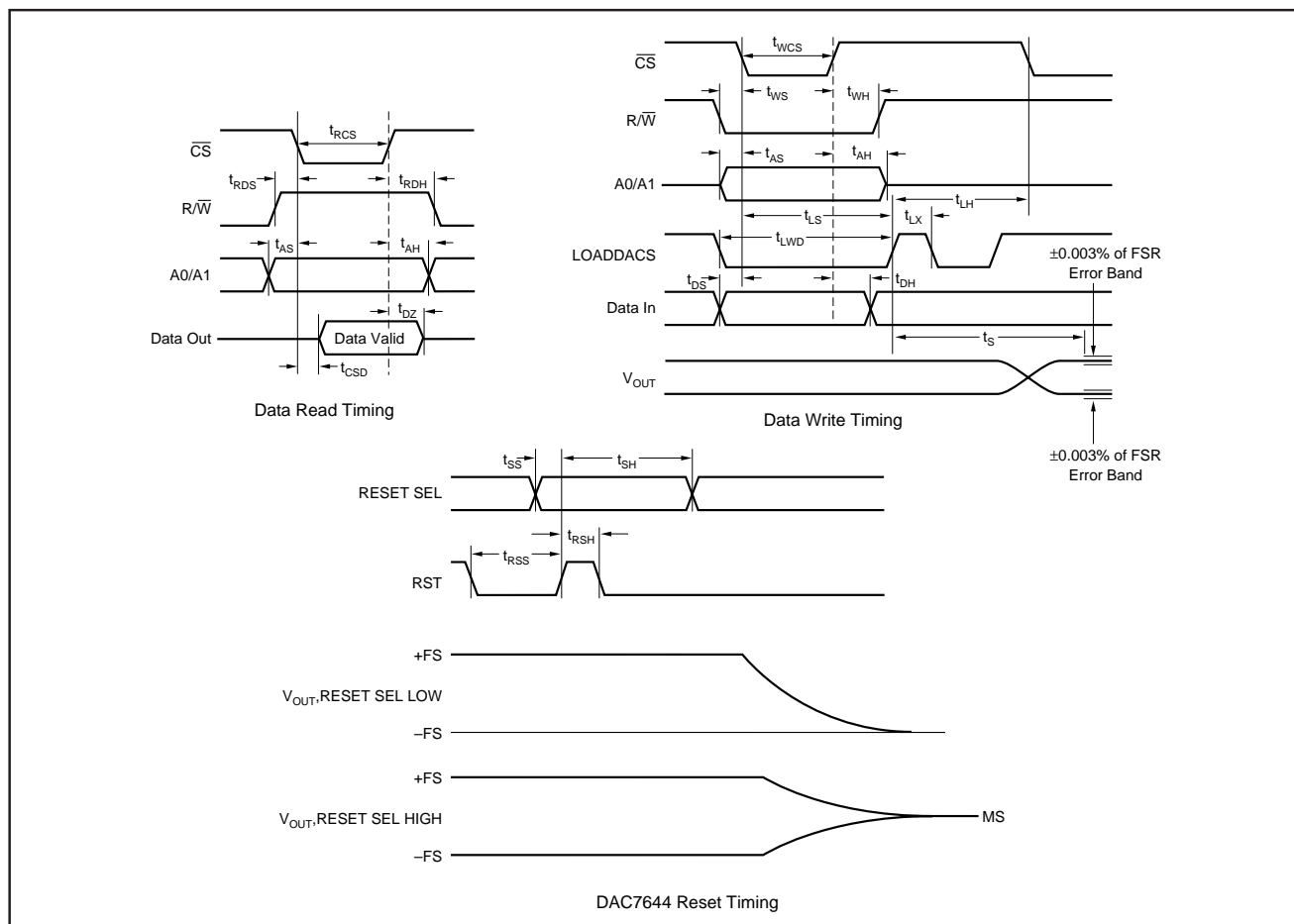
FIGURE 14. Digital Input and Output Timing.
