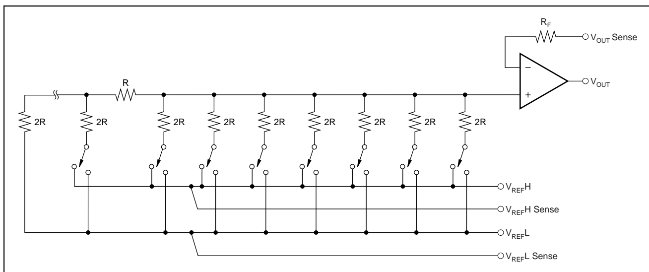
FIGURE 1. DAC7644 Architecture.
