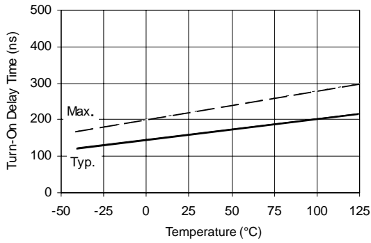
Figure 6A. Turn-On Time vs Temperature
