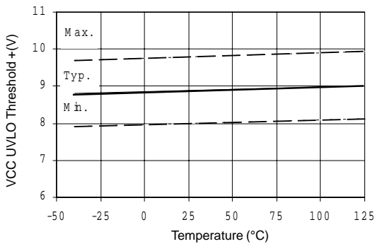
Figure 21A. Vcc Undervoltage Threshold(+) vs Temperature
