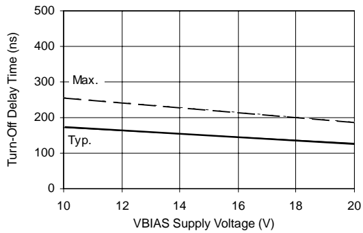
Figure 7B. Turn-Off Time vs Supply Voltage
