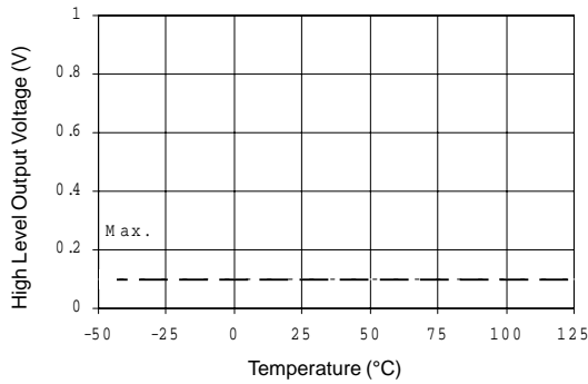
Figure 14A. High Level Output vs Temperature
