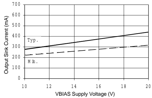
Figure 23B. Output Sink Current vs Voltage
