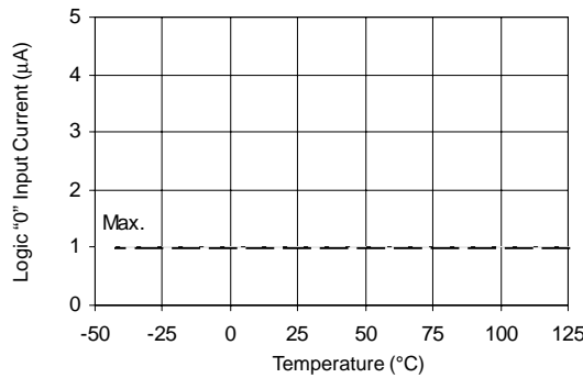
Figure 20A. Logic "0" Input Current vs Temperature
