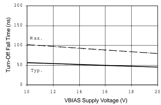
Figure 10B. Turn-Off Fall Time vs Voltage
