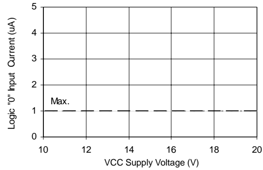
Figure 20B. Logic "0" Input Current vs Voltage
