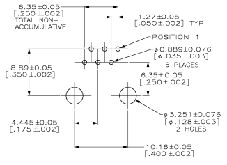
SUGGESTED PC BOARD LAYOUT CIRCUIT SIDE SHOWN
