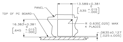
SUGGESTED PANEL CUTOUT SCALE 2:1
