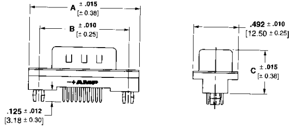
Vertical Plug
