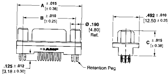
Vertical Receptacle
