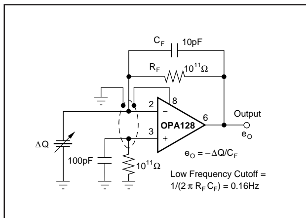
FIGURE 4. Piezoelectric Transducer Charge Amplifier.
