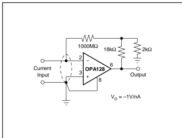
FIGURE 8. Current-to-Voltage Converter.
