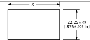
RECOMMENDED PANEL MOUNTING
