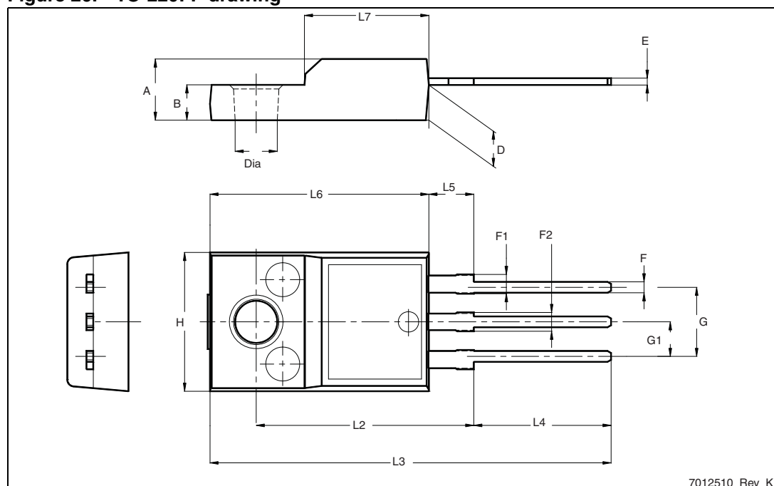
Figure 26. TO-220FP drawing
