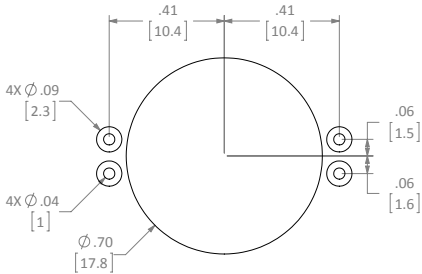
RECOMMENDED FOOTPRINT
