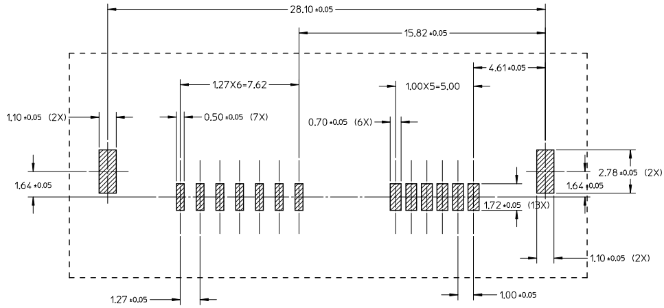
RECOMMENDED PCB LAYOUT DIMENSION
