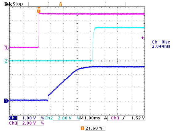
Figure 16: Control Turn on, 2.5V/80A out Ch1: Vo, Ch2:PG, Ch3:Enable
