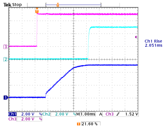
Figure 18: Control Turn on, 5V/80A out Ch1: Vo, Ch2:PG, Ch3:Enable
