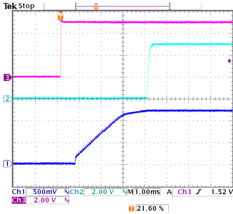
Figure 13: Control Turn on, 1.2V/80A out Ch1: Vo, Ch2:PG, Ch3:Enable
