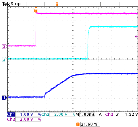
Figure 15: Control Turn on, 1.8V/80A out Ch1: Vo, Ch2:PG, Ch3:Enable
