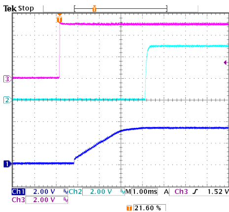
Figure 17: Control Turn on, 3.3V/80A out Ch1: Vo, Ch2:PG, Ch3:Enable
