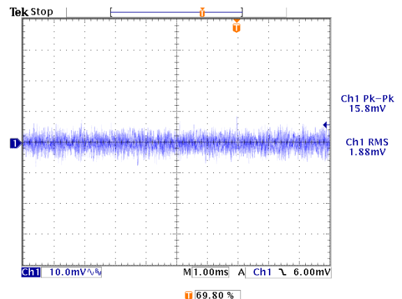
Figure 12: Output ripple & noise at 12Vin, 5.0V/80A out (10mv/div, 1mS/div)
