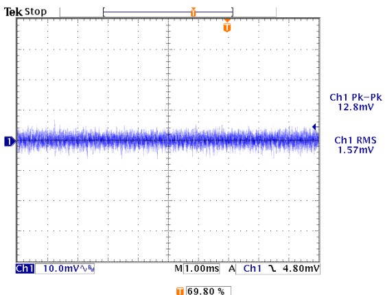
Figure 11: Output ripple & noise at 12Vin, 3.3V/80A out (10mv/div, 1mS/div)
