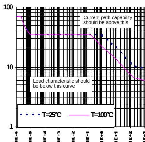
Figure 14 - Max.Cont. Ids (A) Vs Ambient Temperature (°C)
