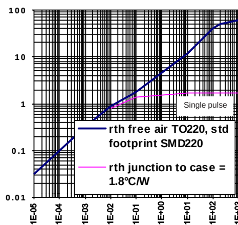
Figure 16 - Transient Thermal Imped. (°C/W) Vs Time (s) - IPS0151/IPS051S
