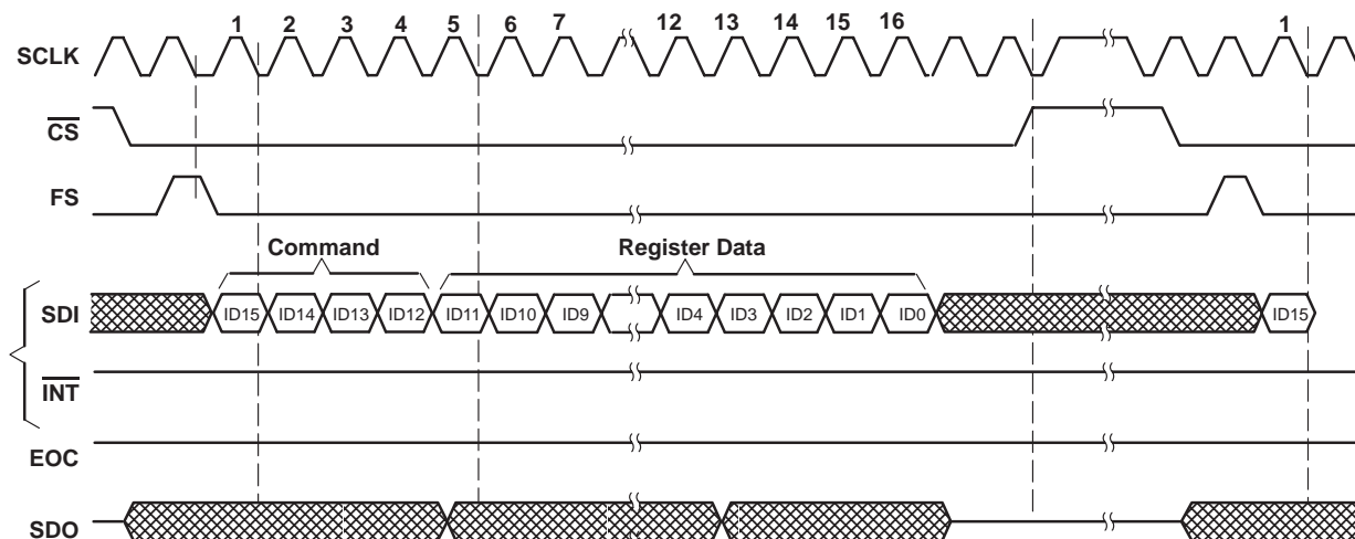
Figure 5. TLC1514/TLC1518 Write Cycle ( \text{FS} active)
