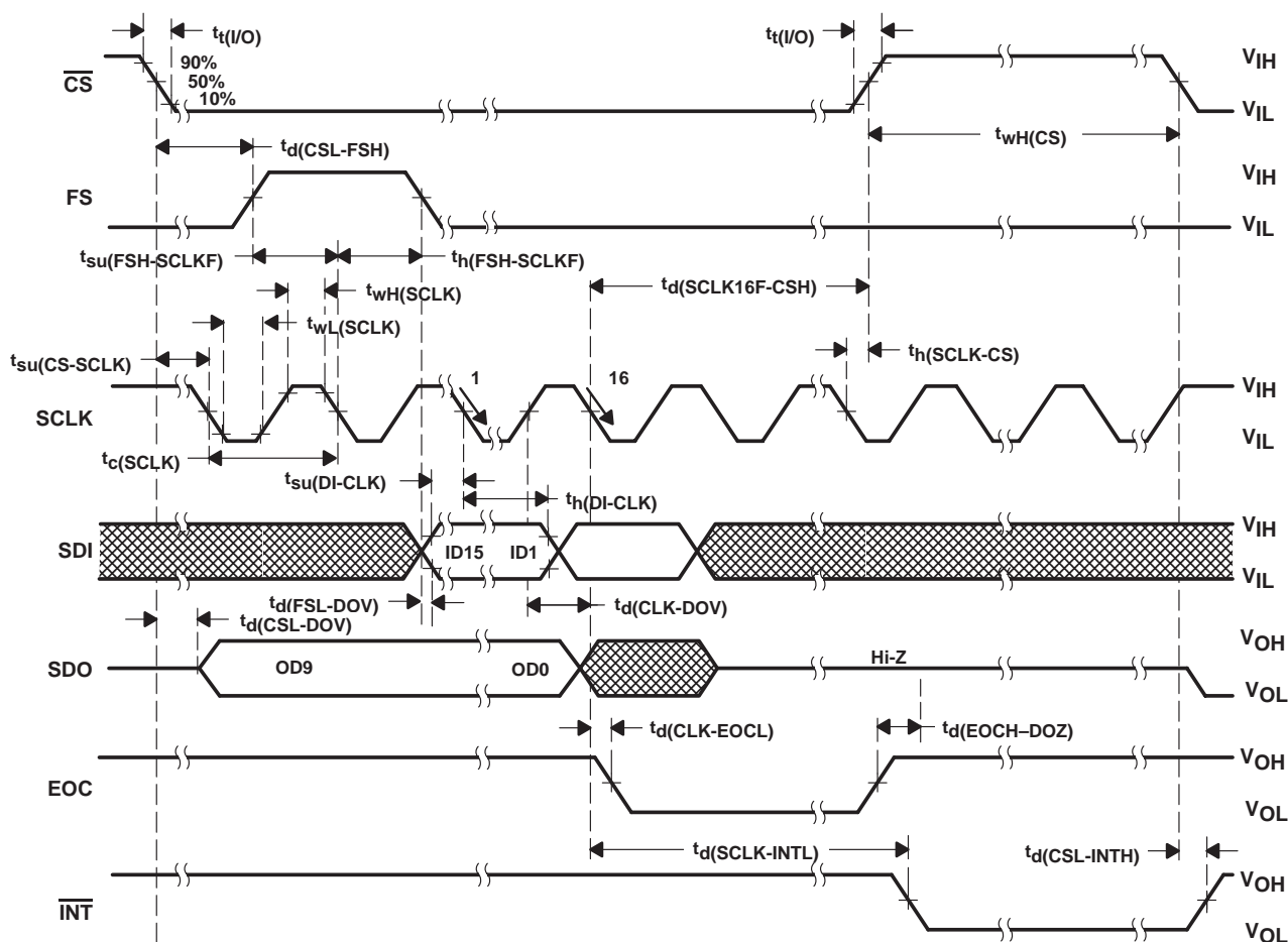
Figure 16. Critical Timing (normal sampling, \overline{\text{FS}} is active)
