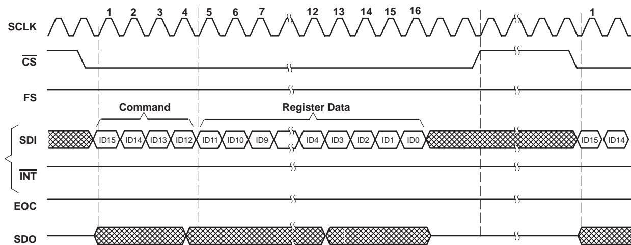
Figure 6. TLC1514/TLC1518 Write Cycle ( \text{FS} = 1 )
