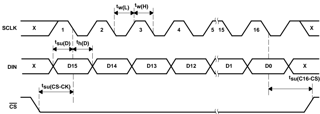
Figure 1. Timing Diagram
