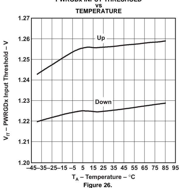
PWRGDx INPUT THRESHOLD
