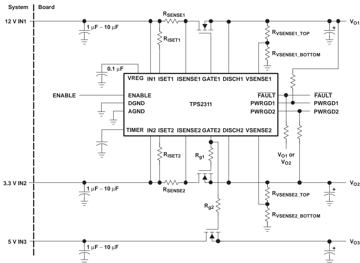
Figure 28. Three-Channel Application
