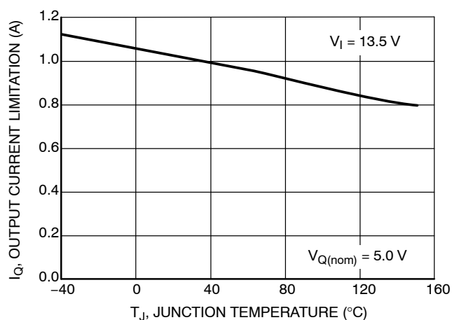
Figure 6. Output Current I_Q vs. Temperature T_J
