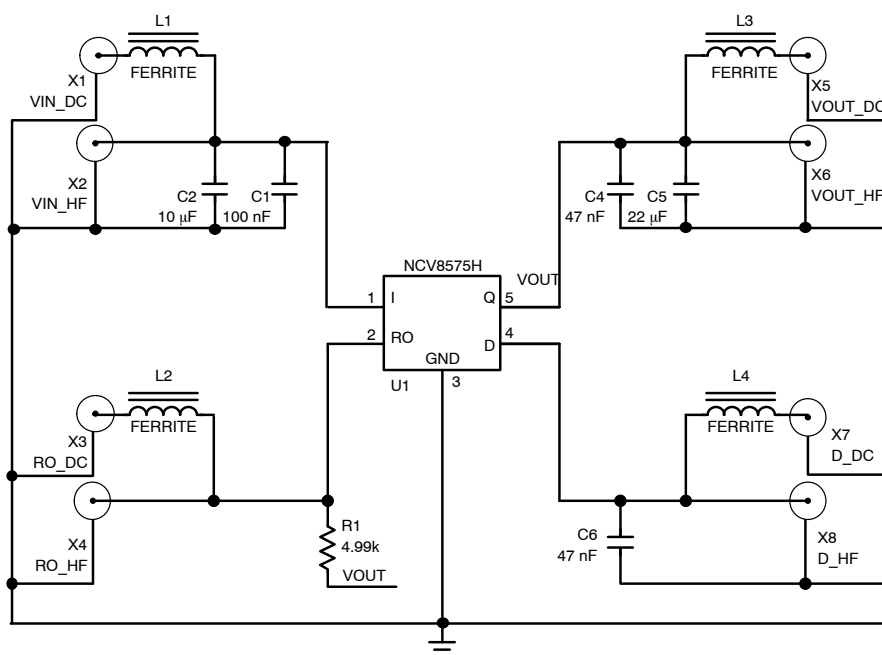
Figure 21. Test Circuit
