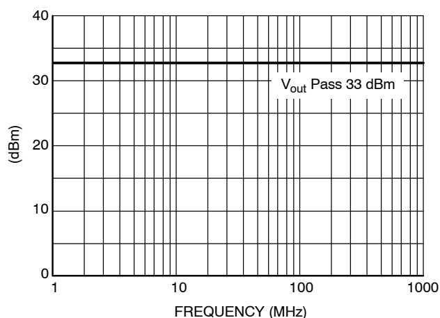
Figure 23. Typical V_{out} Pin Susceptibility
