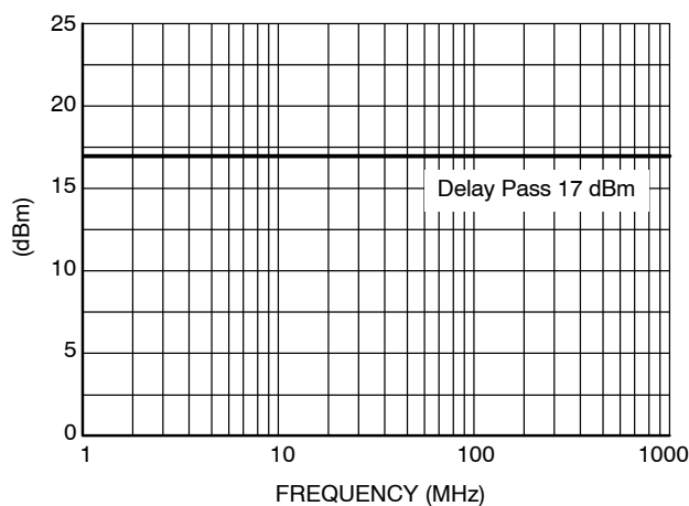
Figure 25. Typical Delay Pin Susceptibility
