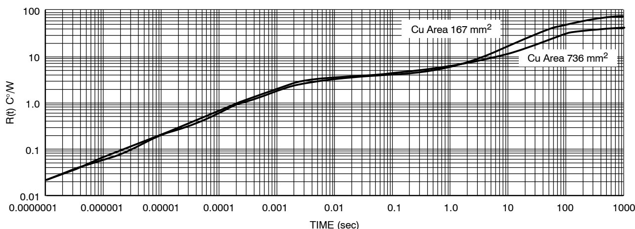
Figure 19. Single-Pulse Heating Curves, D 2 PAK 5-Lead
