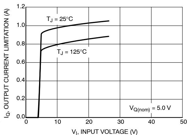
Figure 7. Output Current I_Q vs. Input Voltage V_I
