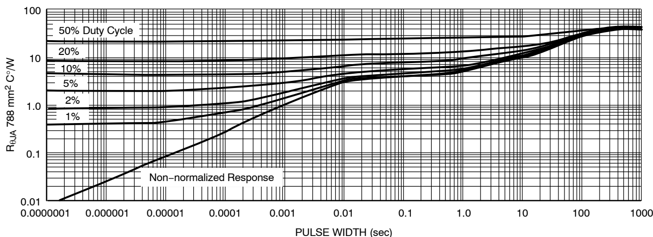
Figure 20. Duty Cycle for 1" Spreader Boards, D 2 PAK 5-Lead
