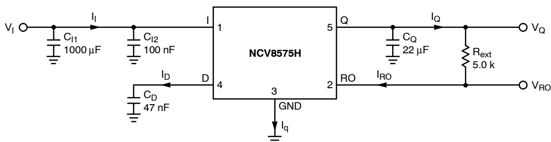
Figure 13. Test Circuit
