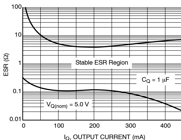
Figure 3. Output Stability with Output Capacitor ESR
