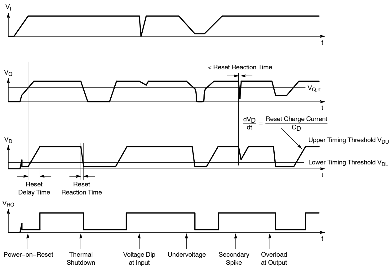
Figure 14. Reset Timing
