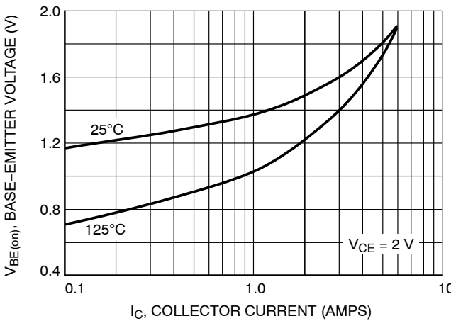
Figure 6. Base-Emitter Voltage
