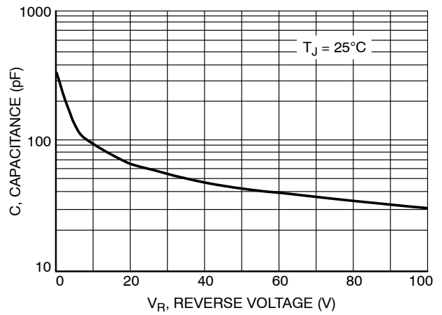
Figure 4. Typical Capacitance
