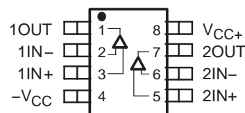
THS4052 D AND DGN† PACKAGES (TOP VIEW)
