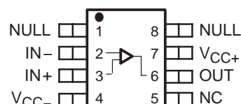
THS4051 D, DGN, AND JG PACKAGES (TOP VIEW)
