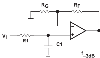
Figure 49. Single-Pole Low-Pass Filter
