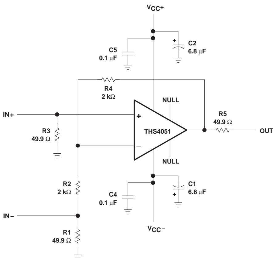
Figure 58. THS4051 Evaluation Board Schematic
