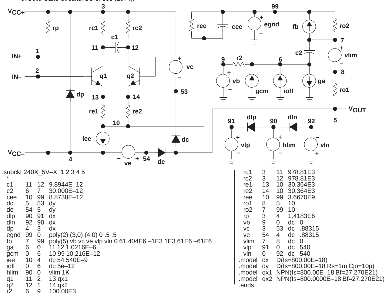
Figure 41. Boyle Macromodels and Subcircuit
