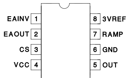
DIL-8, SOIC-8 (TOP VIEW) D, N or J Packages
