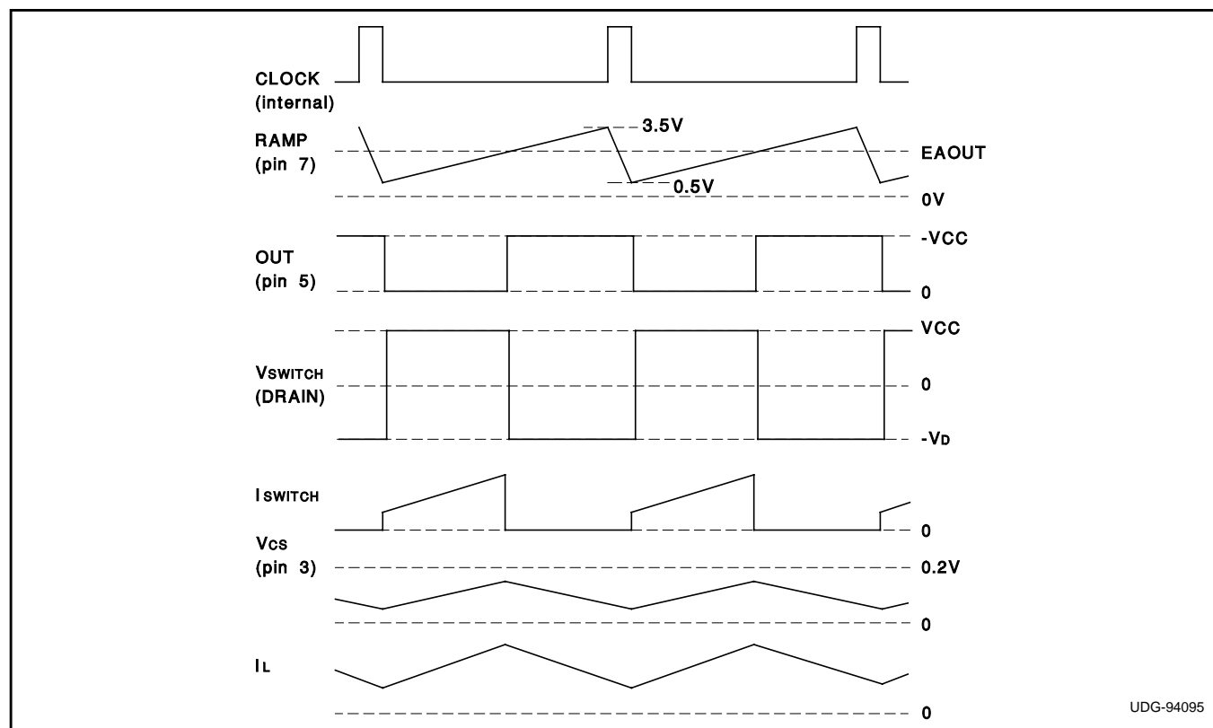
Figure 1. Typical waveforms.
