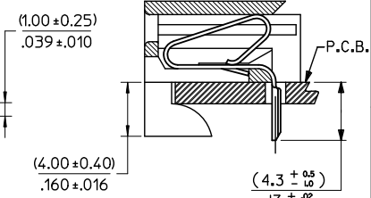
SECTION X-X
