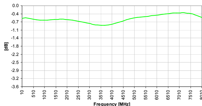
Insertion Loss
