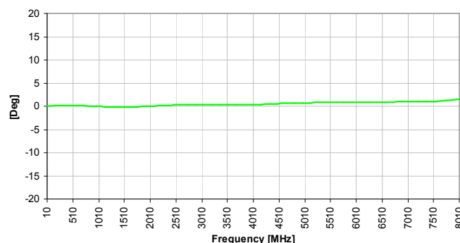
Phase Balance
