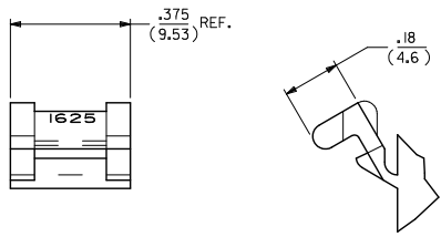
DETAIL B .062/(1.57) PREBENT MOUNTING EAR (SCALE 4:1)
