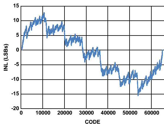
FIGURE 11. INTEGRAL NONLINEARITY
