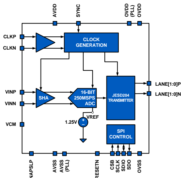
FIGURE 2. BLOCK DIAGRAM
