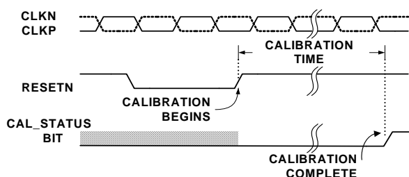
FIGURE 29. CALIBRATION TIMING
