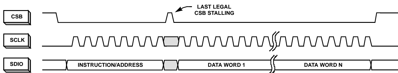
FIGURE 47. N-BYTE TRANSFER
