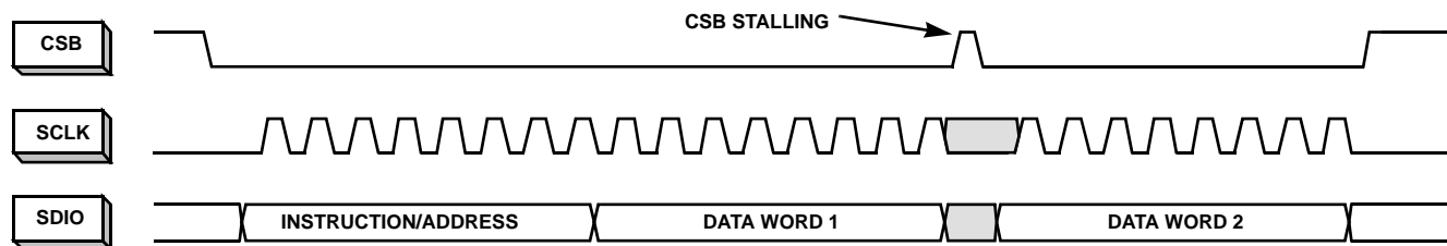
FIGURE 46. 2-BYTE TRANSFER
