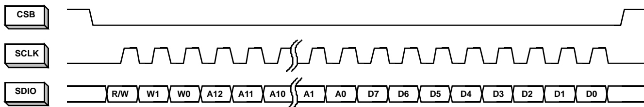
FIGURE 42. MSB-FIRST ADDRESSING
