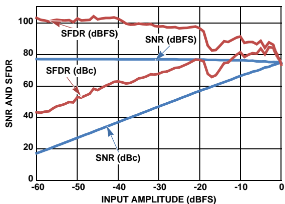
FIGURE 5. SNR AND SFDR vs AIN
