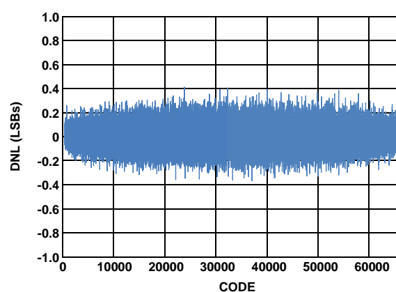
FIGURE 10. DIFFERENTIAL NONLINEARITY
