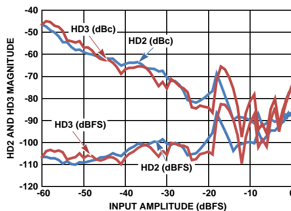
FIGURE 6. HD2 AND HD3 vs AIN
