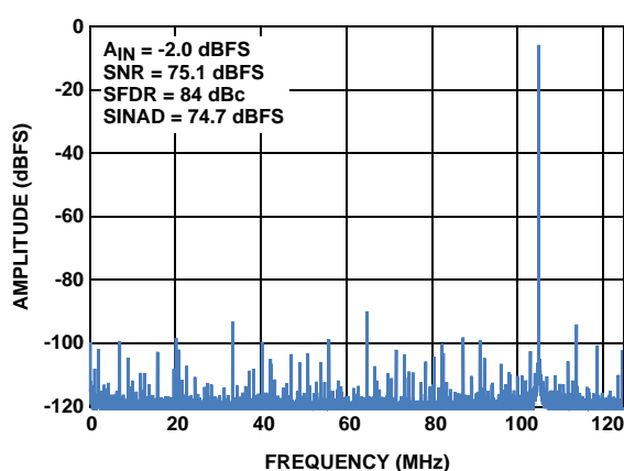
FIGURE 14. SINGLE-TONE SPECTRUM @ 105MHz
