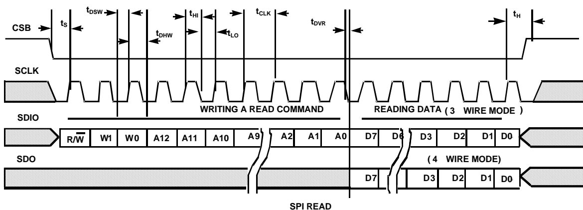
SPI READ
