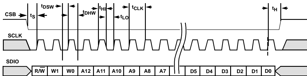
SPI WRITE
