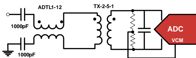
FIGURE 35. TRANSMISSION-LINE TRANSFORMER INPUT FOR HIGH IF APPLICATIONS
