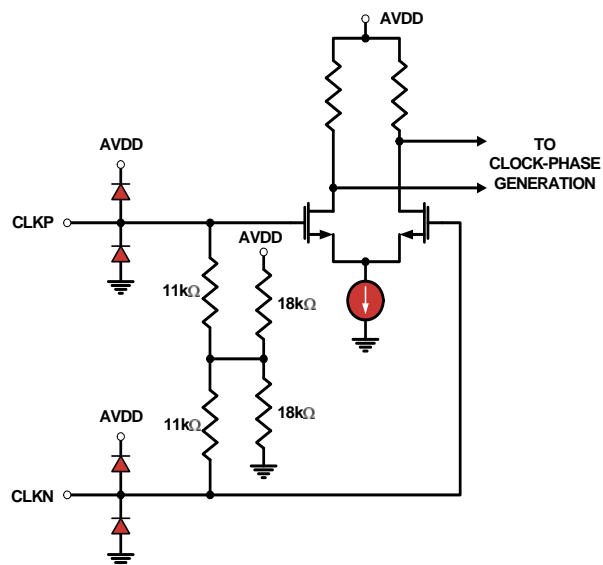
FIGURE 49. CLOCK INPUTS
