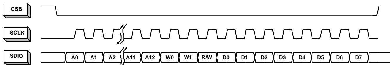
FIGURE 43. LSB-FIRST ADDRESSING
