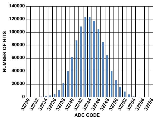
FIGURE 13. NOISE HISTOGRAM
