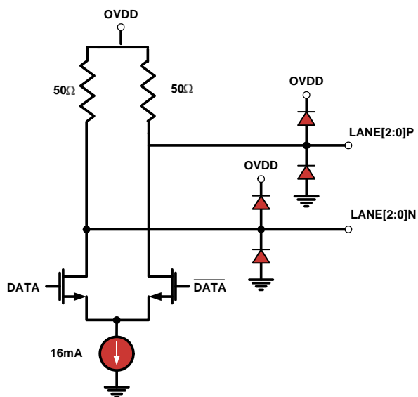
FIGURE 52. CML OUTPUTS
