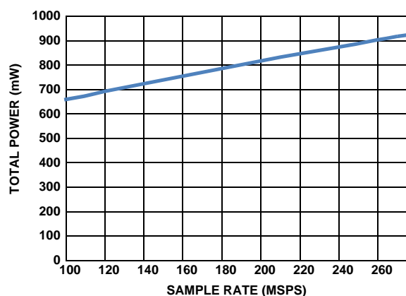
FIGURE 9. POWER vs fSAMPLE
