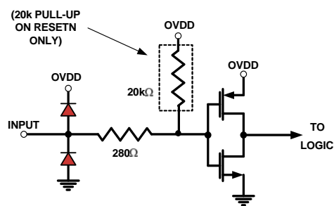
FIGURE 51. DIGITAL INPUTS
