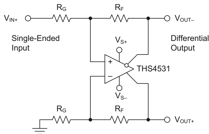
Figure 75. Single-Ended Input to Differential Output Amplifier
