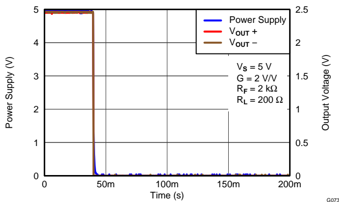
Figure 84. Power Supply Turn Off Pop Performance
