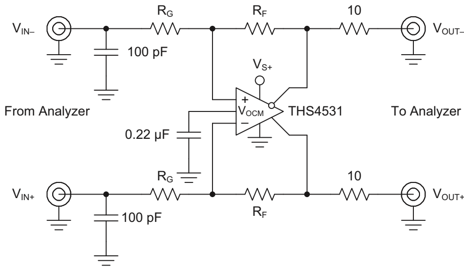
Figure 80. THS4531 Audio Analyzer Test Circuit
