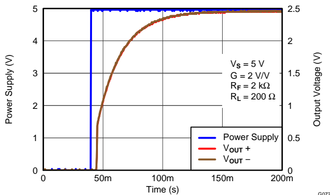
Figure 83. Power Supply Turn On Pop Performance
