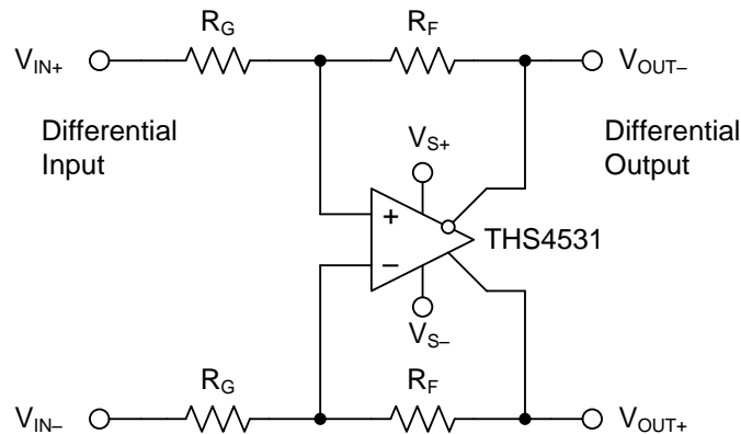
Figure 74. Differential Input to Differential Output Amplifier
