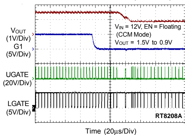
V OUT Down Transient (No Load)
