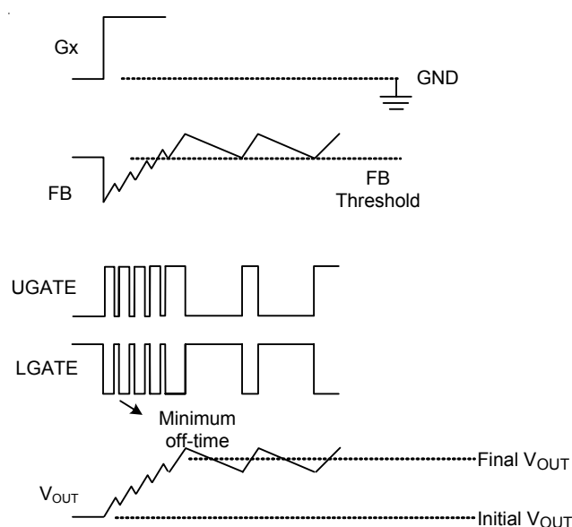
Figure 5. Output Voltage Up Transition
