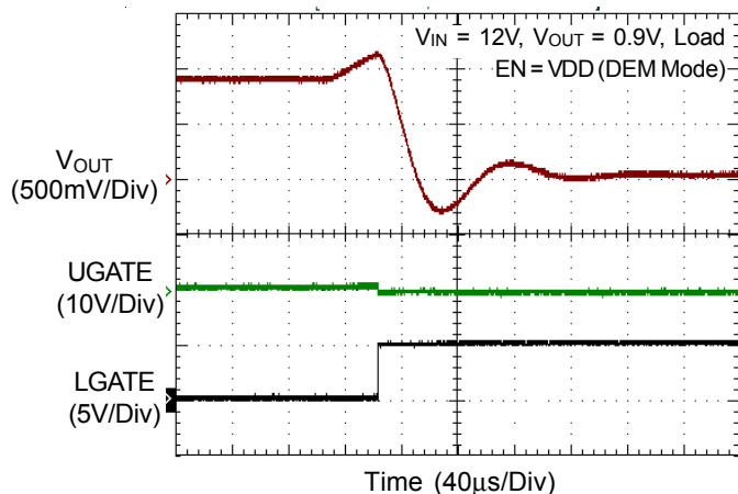
OVP Waveforms
