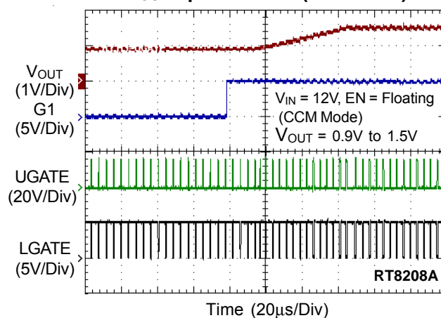
V OUT Up Transient (Load=10A)
