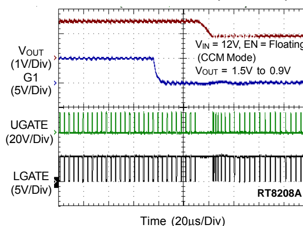
V OUT Down Transient (Load=10A)
