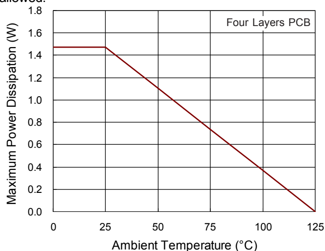
Figure 9. Derating Curve for RT8208A/B Package
