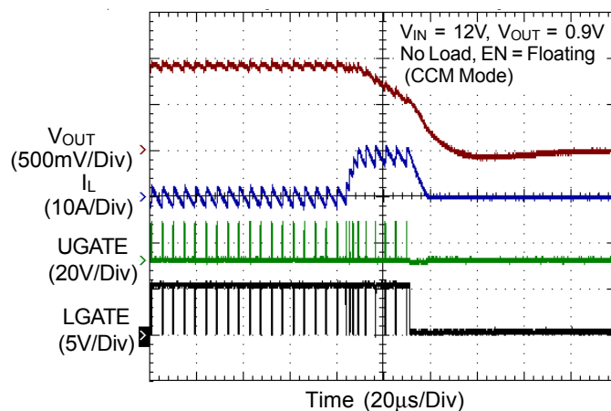
UVP Waveforms
