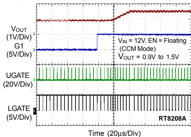
V OUT Up Transient (No Load)
