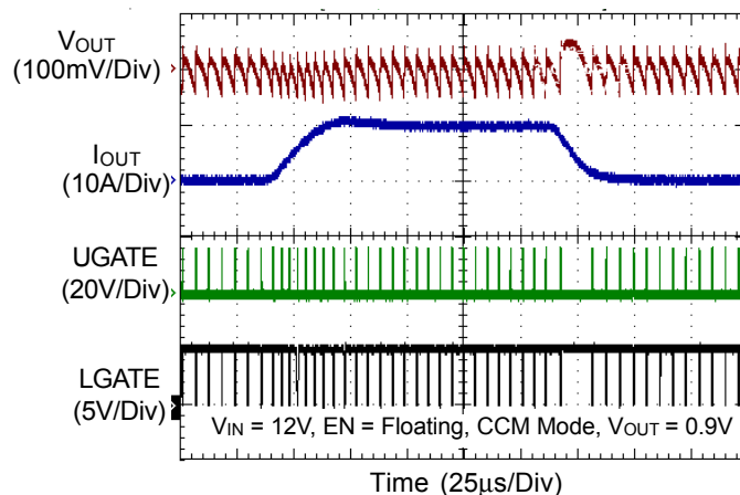
0.9V Load Transient Response
