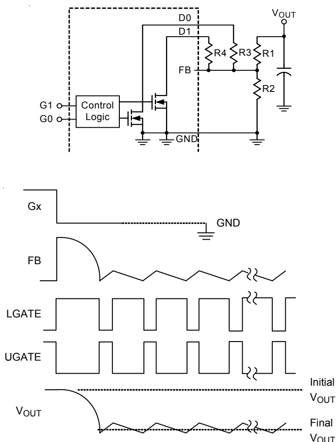
Figure 4. Output Voltage Down Transition
