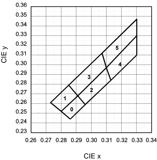
[Chromaticity Coordinates] (Ta=25°C, I F =90mA)
