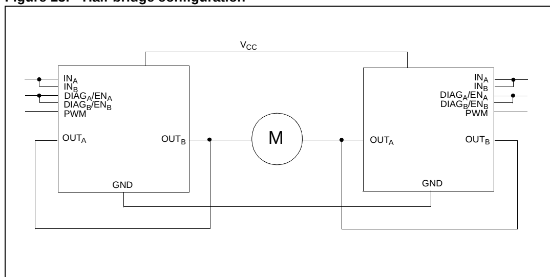
Figure 13. Half-bridge configuration
