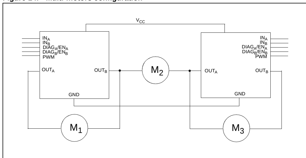
Figure 14. Multi-motors configuration
