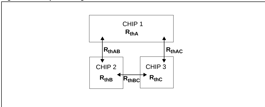
Figure 16. Chipset configuration
