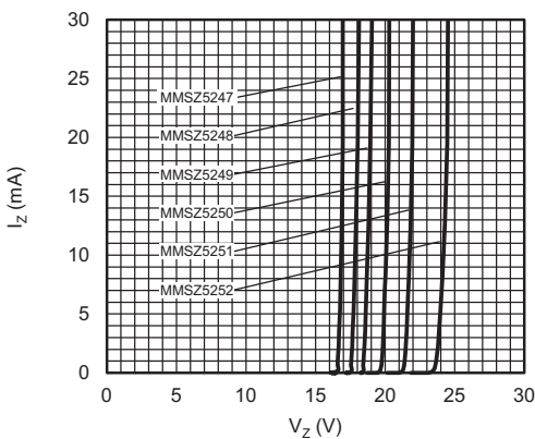
Fig. 3 - Breakdown Characteristics
