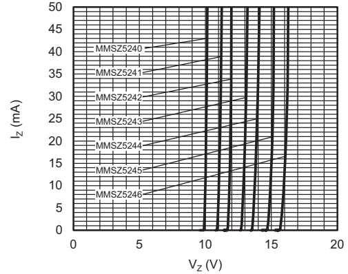
Fig. 4 - Breakdown Characteristics
