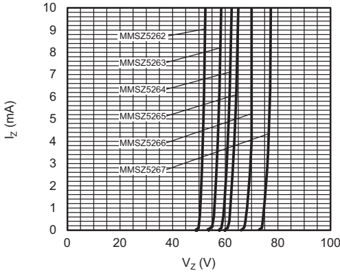
Fig. 1 - Breakdown Characteristics
