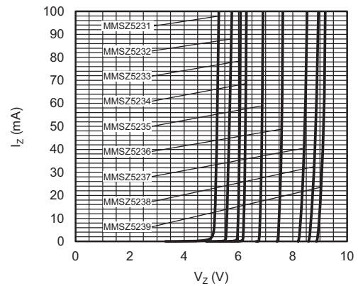
Fig. 5 - Breakdown Characteristics
