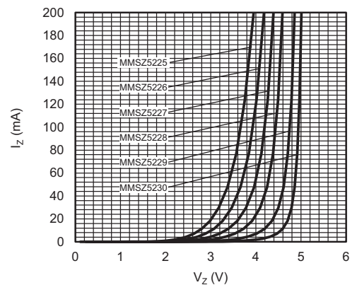
Fig. 6 - Breakdown Characteristics
