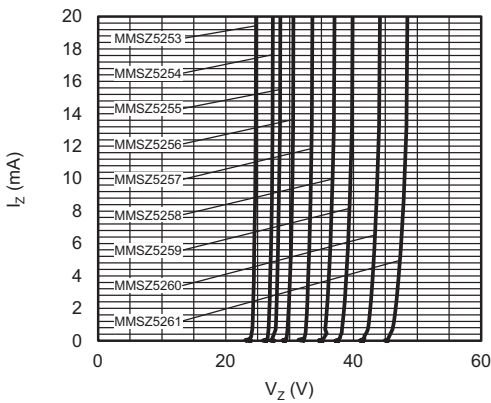
Fig. 2 - Breakdown Characteristics
