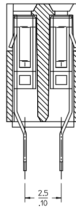
SECTION C-C
