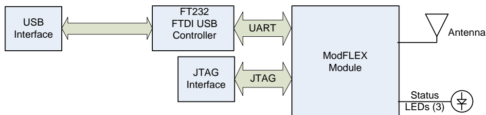
Figure 1 Mini Gateway USB Block Diagram – High-Level
