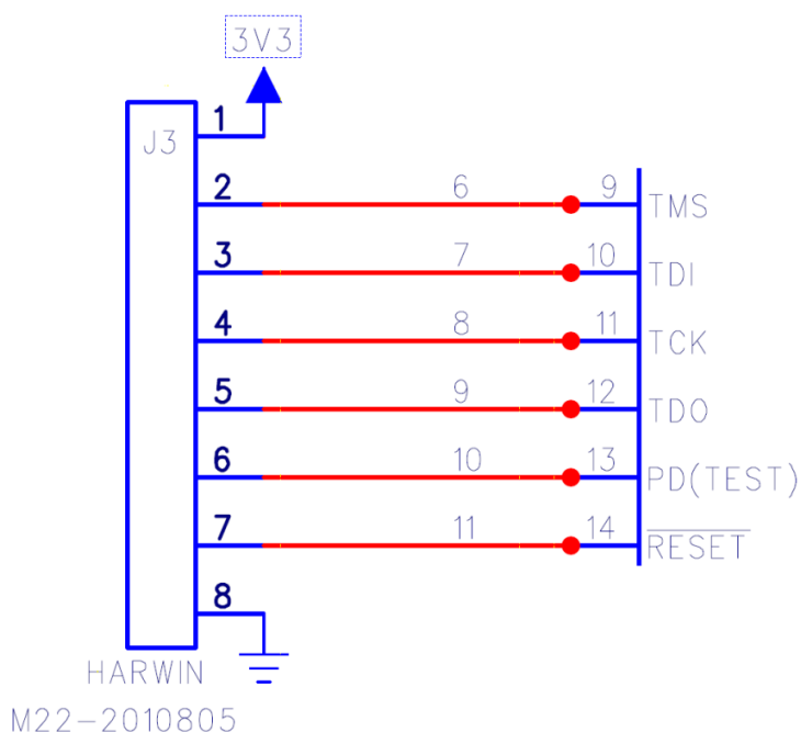
Figure 3 Programming Header Schematic
