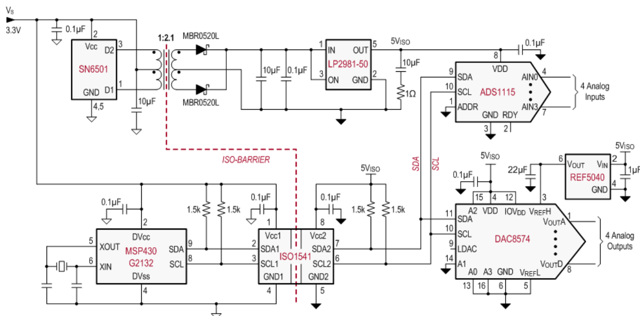
Figure 55. Isolated I²C Interface for an Analog Data Acquisition System With 4 Inputs and 4 Outputs
