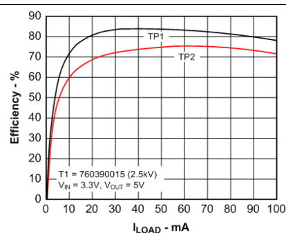
Figure 10. Efficiency vs Load Current
