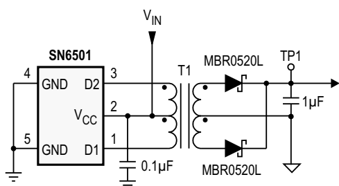
Figure 33. Measurement Circuit for Unregulated Output (TP1)
