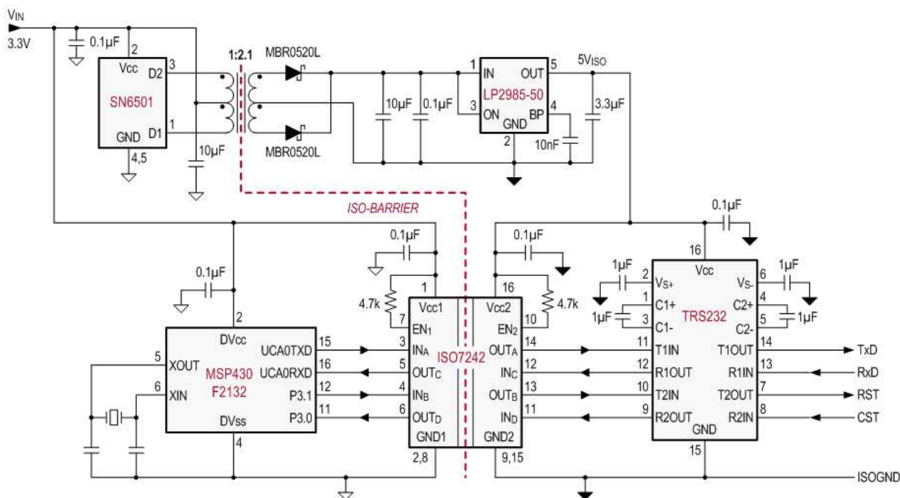
Figure 52. Isolated RS-232 Interface
