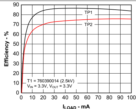
Figure 8. Efficiency vs Load Current
