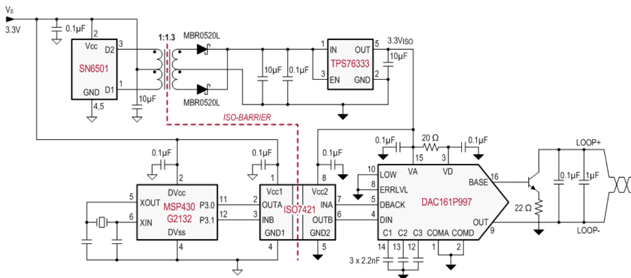
Figure 56. Isolated 4-20 mA Current Loop
