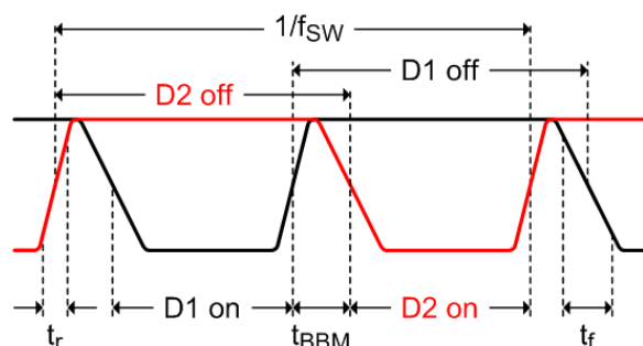
Figure 34. Timing Diagram
