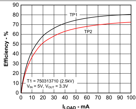
Figure 14. Efficiency vs Load Current
