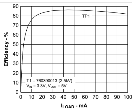
Figure 4. Efficiency vs Load Current
