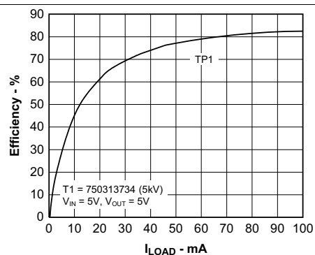
Figure 16. Efficiency vs Load Current
