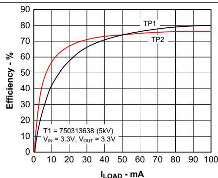
Figure 20. Efficiency vs Load Current
