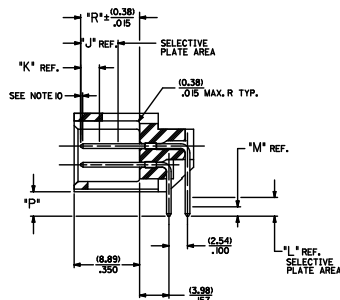
SECTION J-J
