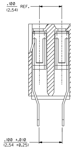
SECTION E-E
