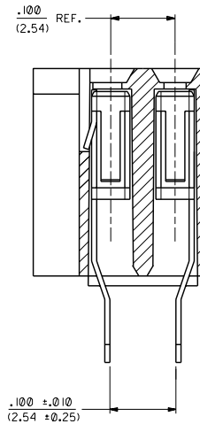
SECTION E-E
