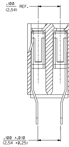
SECTION E-E
