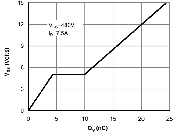
Figure 8: Gate-Charge Characteristics
