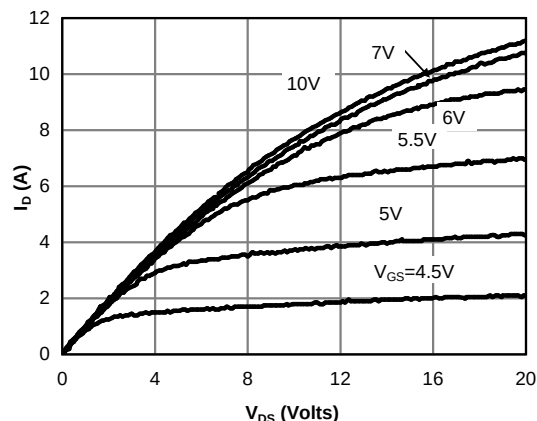
Figure 2: On-Region Characteristics@125°C
