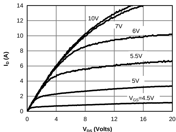
Figure 1: On-Region Characteristics@25°C
