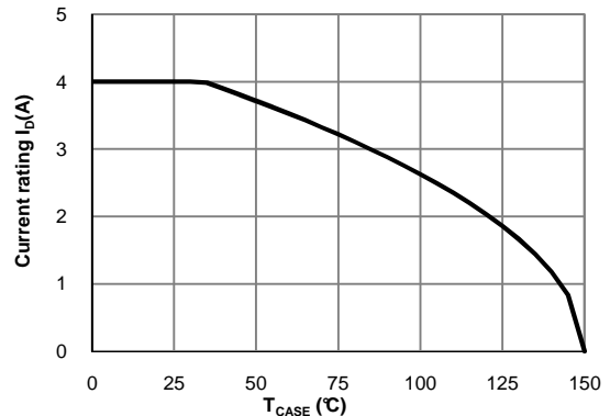
Figure 13: Current De-rating (Note B)
