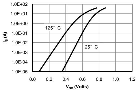
Figure 6: Body-Diode Characteristics (Note E)
