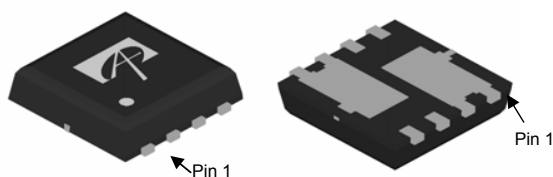
DFN 3x3A_Dual Top View Bottom View
